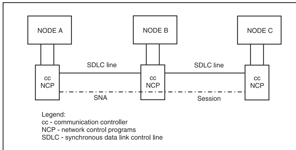
Figure 51. Simple SNA NJE Configuration
