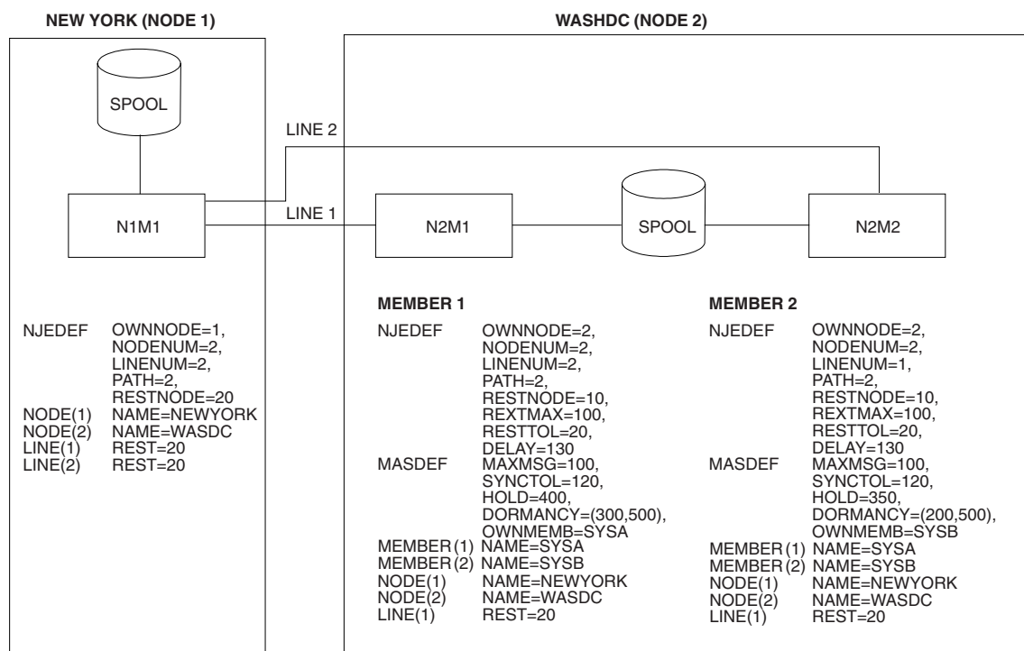
Figure 76. Multi-Access Spool Configuration (BSC)
