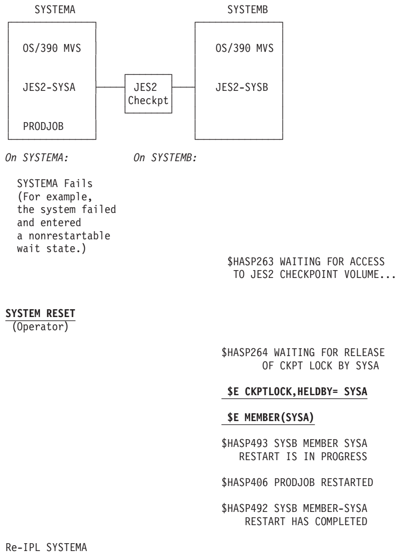
Figure 46. Two-Member MAS with JES2 and MVS Failure (DASD)
