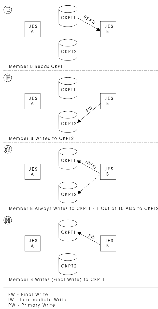
Figure 40. Checkpoint Data Set Processing, DUPLEX Mode, Two-Member Multi-Access Spool Configuration - JESB Cycle
