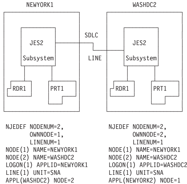
Figure 61. Minimum NJE Configuration (SNA)
