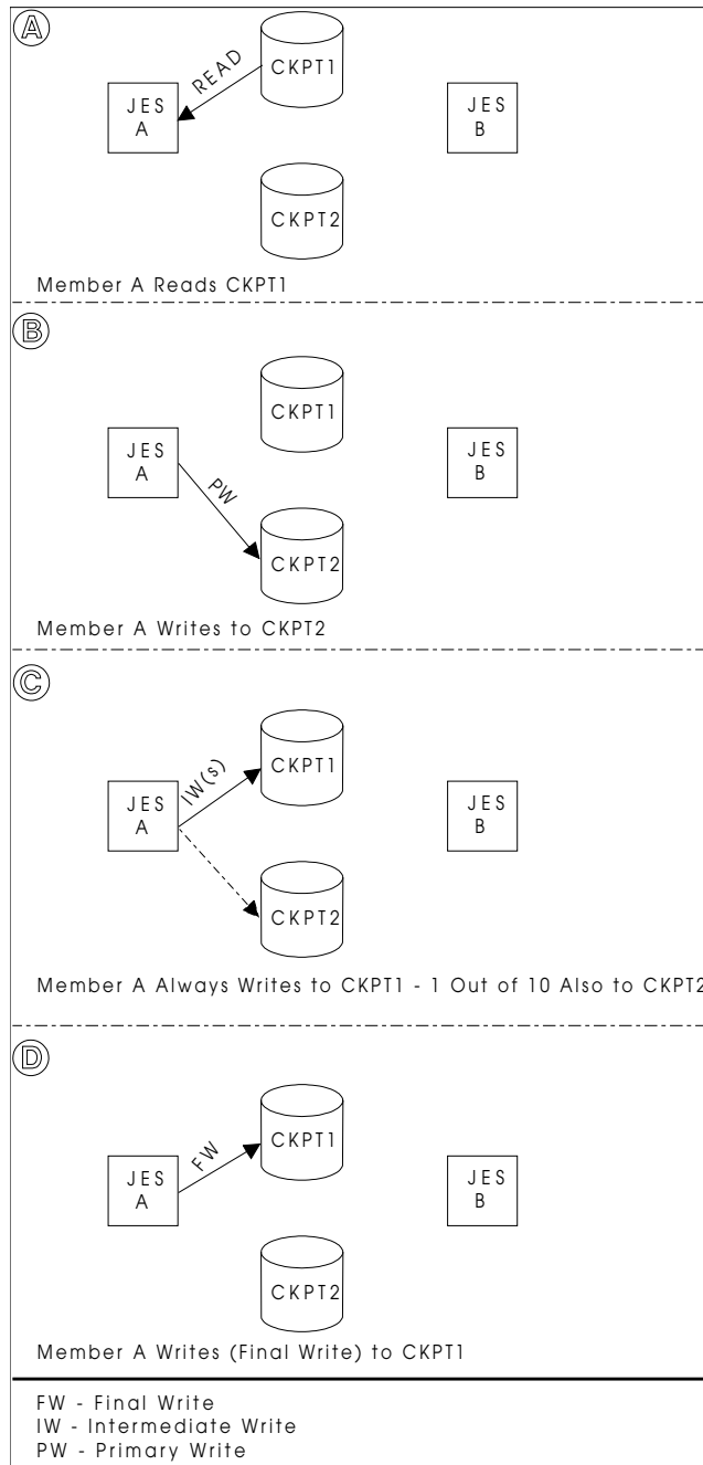
Figure 39. Checkpoint Data Set Processing, DUPLEX Mode, Two-Member Multi-Access Spool Configuration - JESA Cycle
