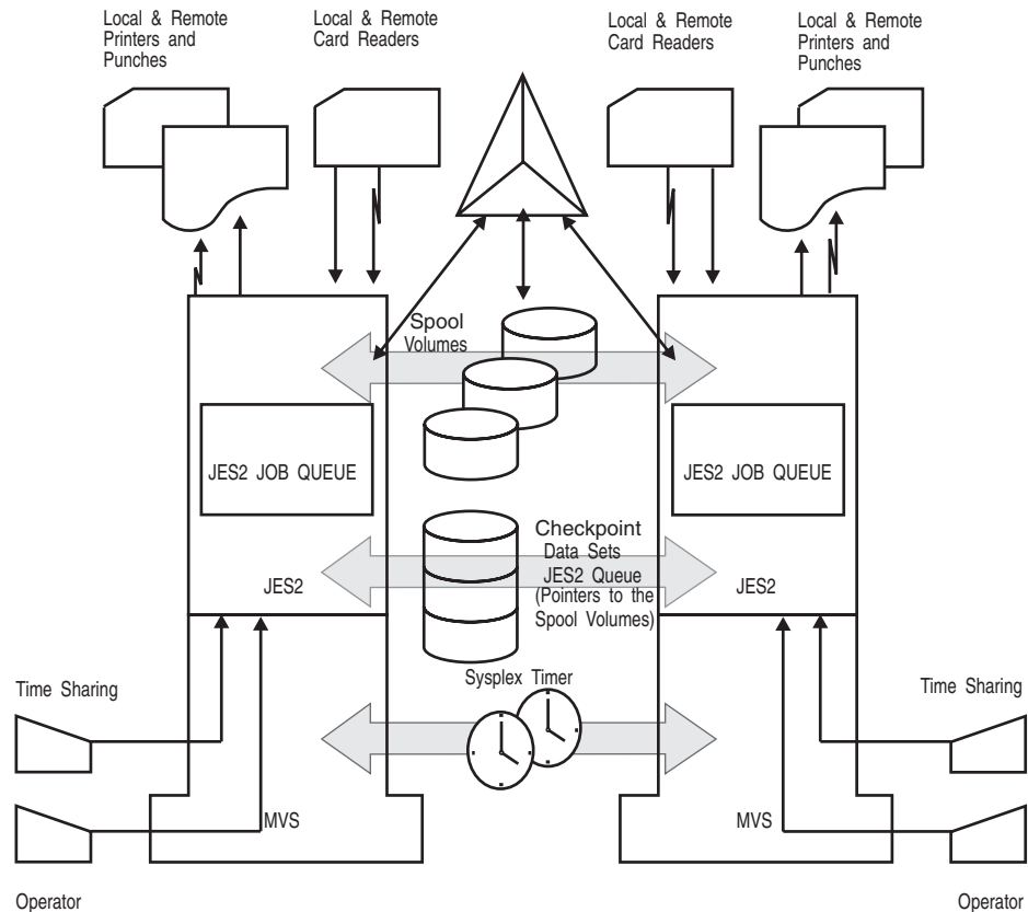
Figure 3. Example of a Two-Member Shared JES2 Configuration
