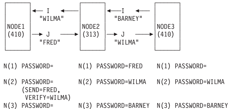
Figure 58. NJE Sign-On Password Verification for Mixed Levels of JES2
