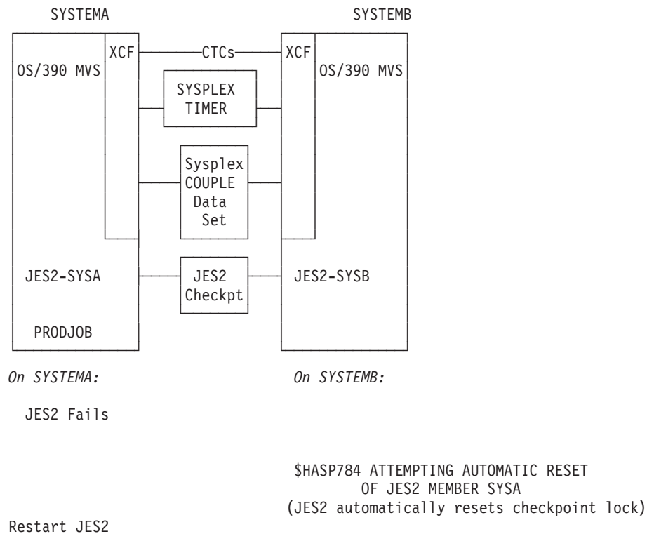
Figure 48. Sysplex with the AUTOEMEM Option Enabled, a JES2 Failure (Coupling Facility)
