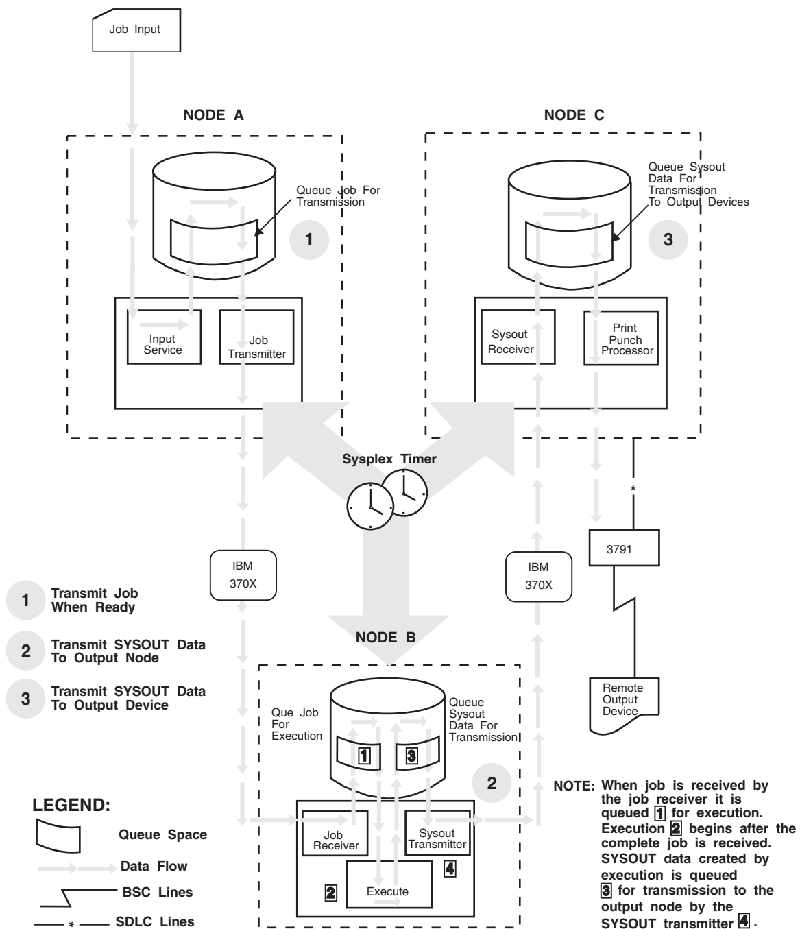
Figure 52. Processing Flow Through a Network
