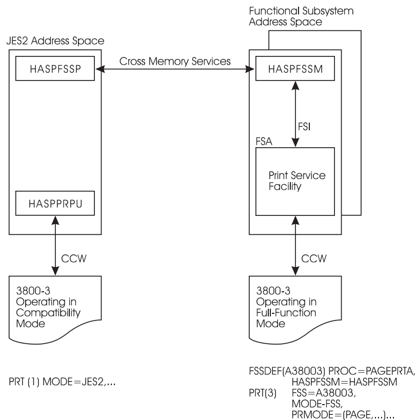
Figure 5. Representation of the Relationship between Functional Subsystem Components
