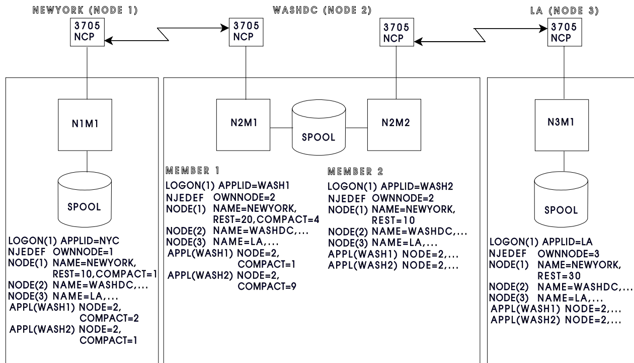
Figure 77. Multi-Access Spool Configuration (SNA)
