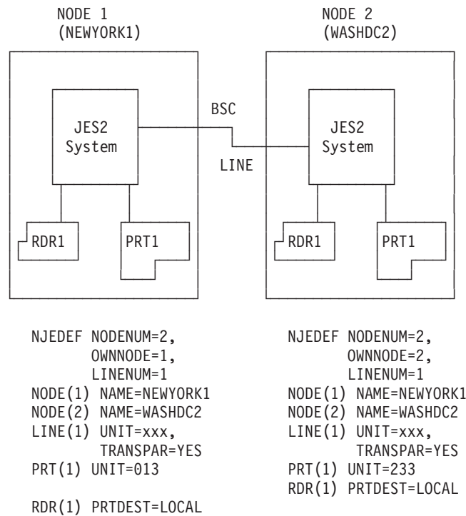
Figure 59. Minimum NJE Configuration (BSC only)
