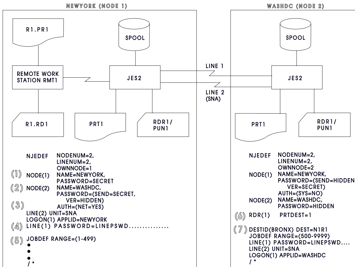
Figure 75. An Expanded Network
