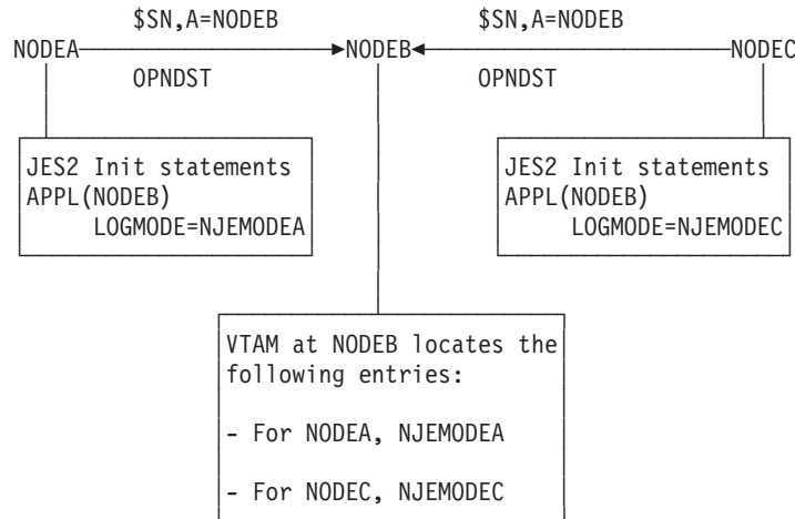
Figure 64. Using Multiple SNA Log Mode Table Entries
